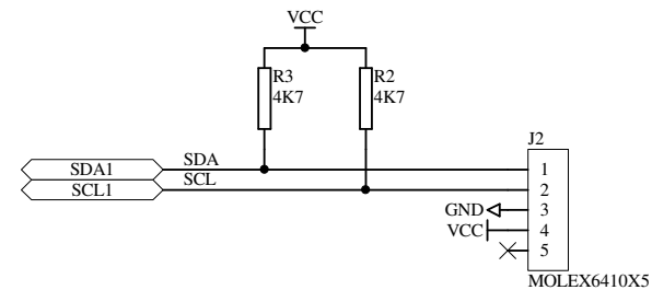
IIC Bus 1
