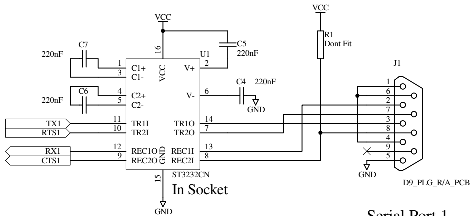
Serial Port 1
